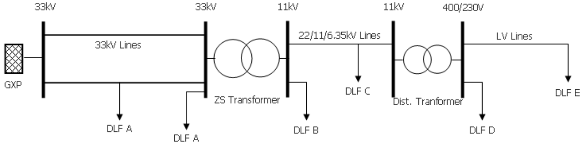
Figure 1: DLF Application at Different Network Stages
